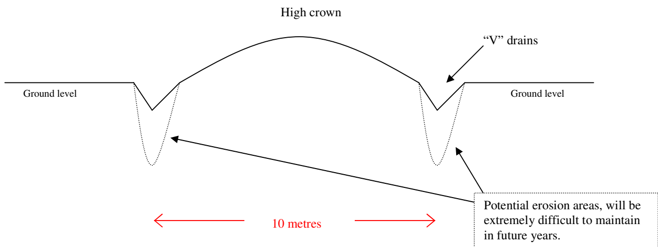
Diagram 1: Road formed too narrow, with no drainage.
