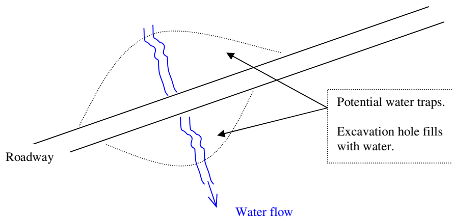
Diagram 2: Formed roads across watercourses.
